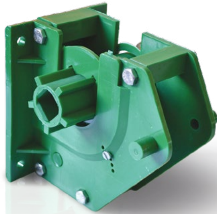
5-GROOVE SEED ROLLER
